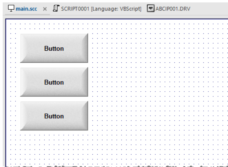
Screen/Worksheet Editor
