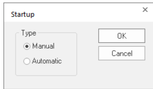
Startup dialog
