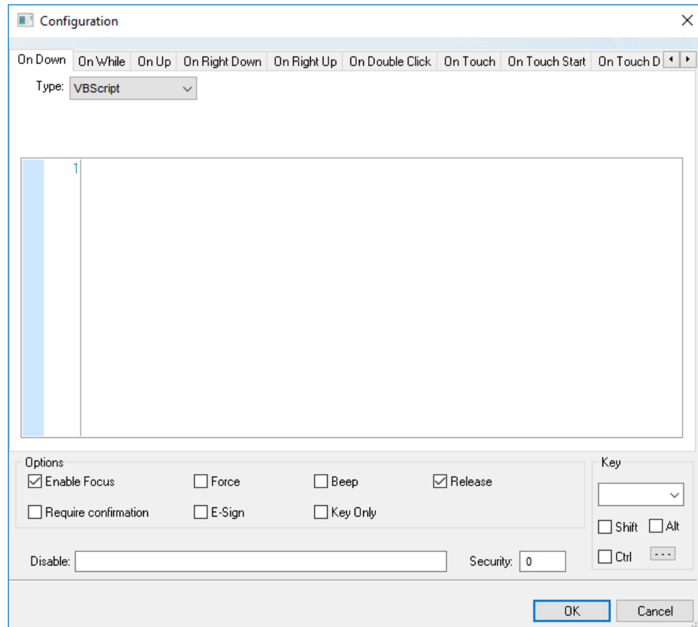
Configuration dialog
