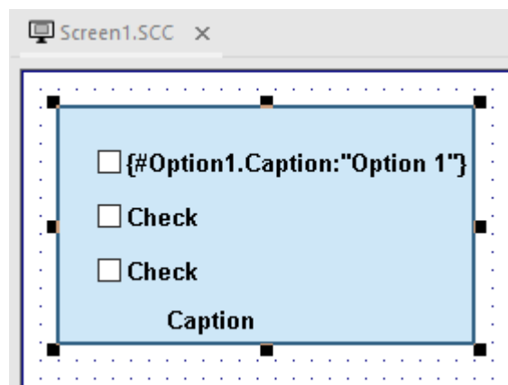
Updated Symbol
