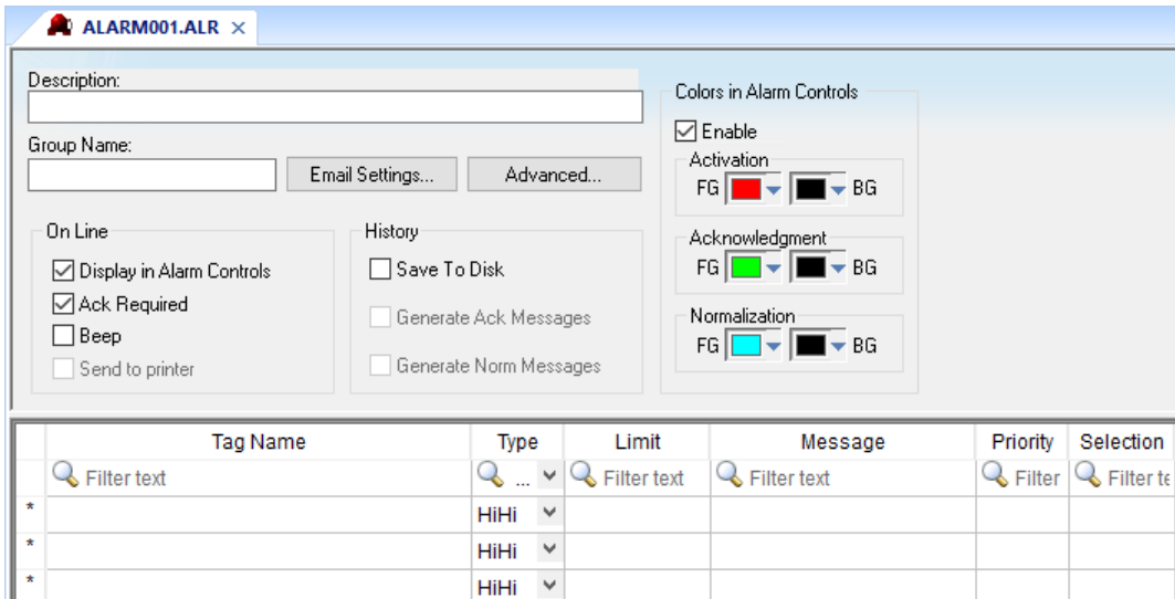
Alarm worksheet
