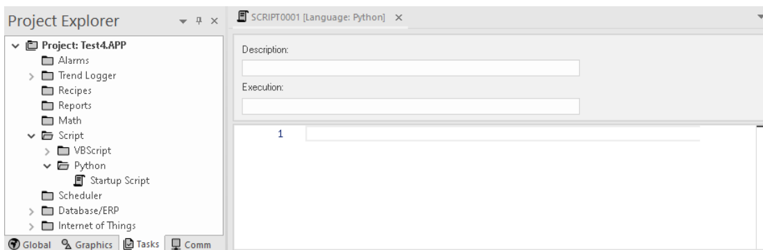
Script worksheet
