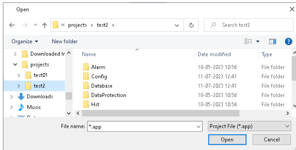
Open dialog
