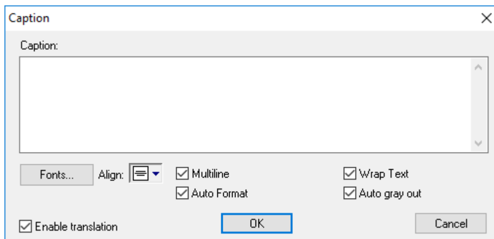
Caption dialog
