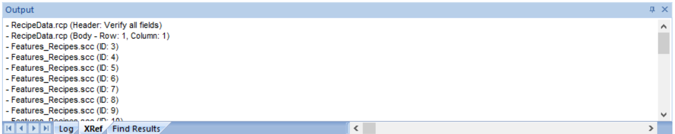
XRef Results
