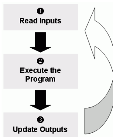
PLC Program Loop
