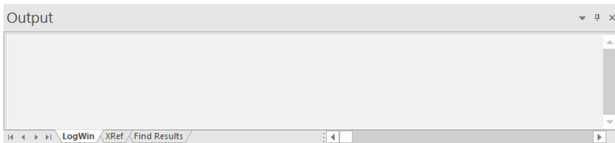
Output window
