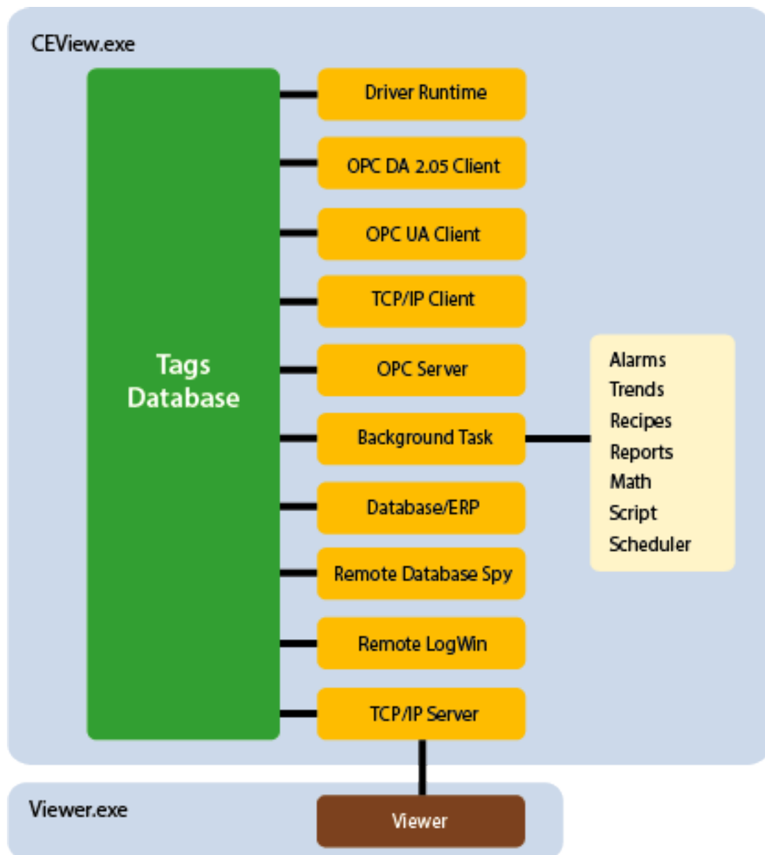
Architecture of the project runtime on Windows Embedded
