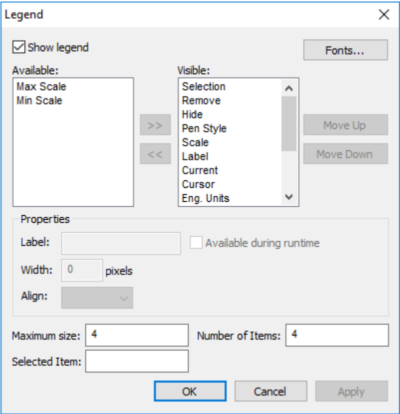
Legend dialog
