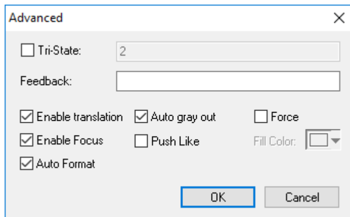
Advanced dialog
