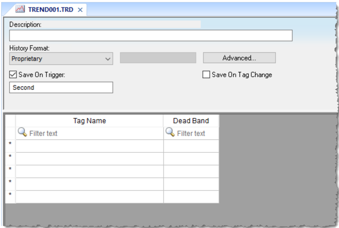
Trend worksheet
