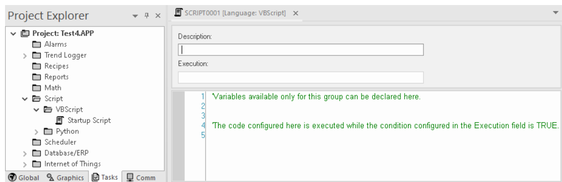
Script worksheet
