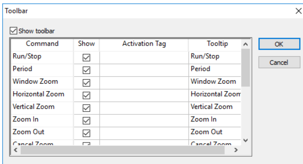
Toolbar dialog
